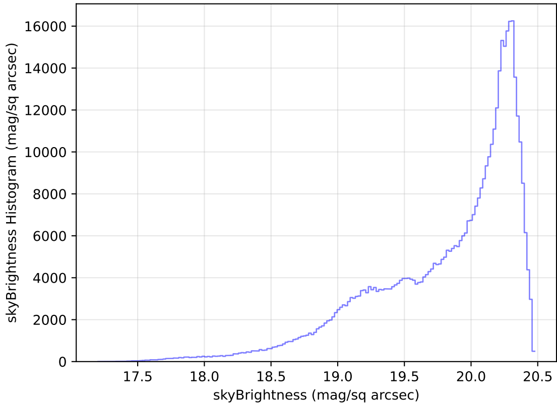
too_elab_r8_d3_giz_v3.4_10yrs All sky i band: skyBrightness Histogram
