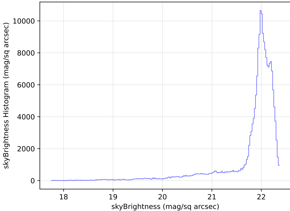
too_elab_r8_d3_giz_v3.4_10yrs All sky g band: skyBrightness Histogram
