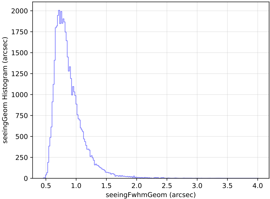
too_elab_r8_d3_giz_v3.4_10yrs Yr 1 z band: seeingGeom Histogram
