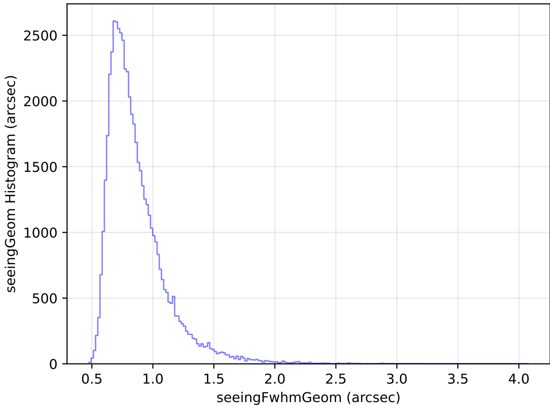
too_elab_r8_d3_giz_v3.4_10yrs Yr 1 i band: seeingGeom Histogram
