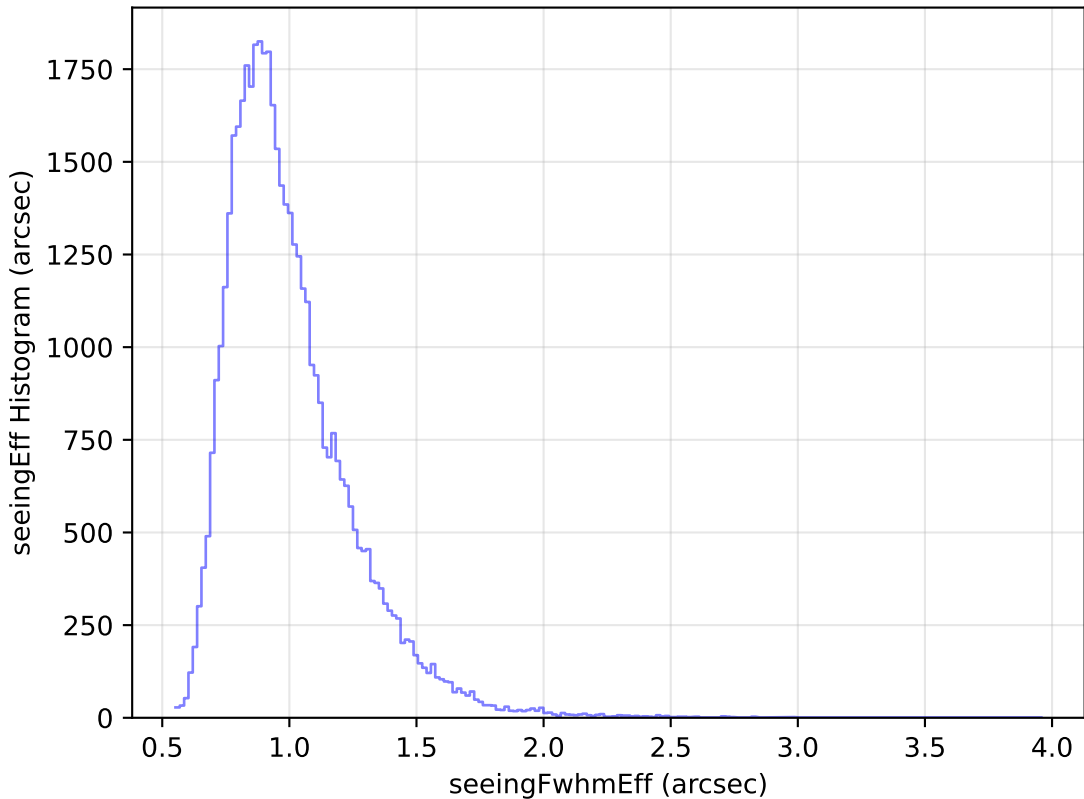
too_elab_r8_d3_giz_v3.4_10yrs Yr 1 y band: seeingEff Histogram
