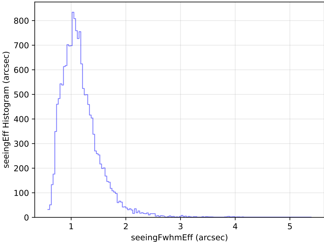
too_elab_r8_d3_giz_v3.4_10yrs Yr 1 u band: seeingEff Histogram
