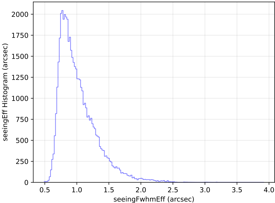
too_elab_r8_d3_giz_v3.4_10yrs Yr 1 r band: seeingEff Histogram
