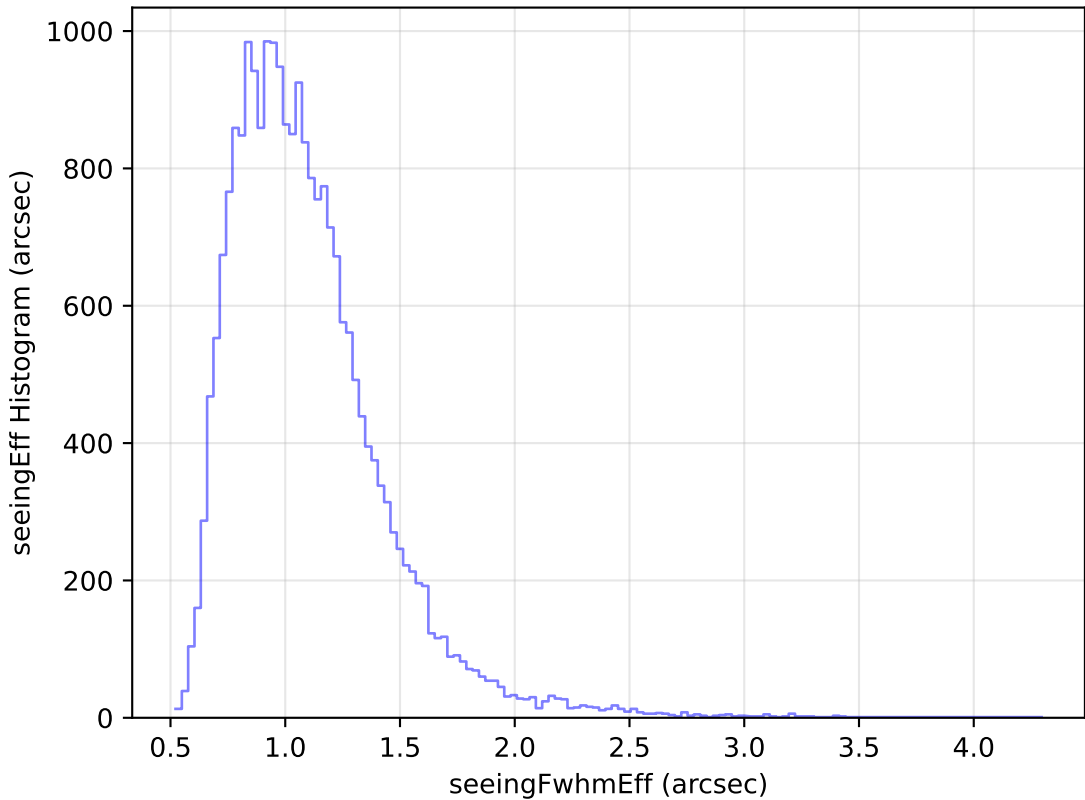
too_elab_r8_d3_giz_v3.4_10yrs Yr 1 g band: seeingEff Histogram
