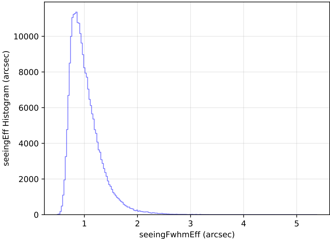
too_elab_r8_d3_giz_v3.4_10yrs Yr 1 all bands: seeingEff Histogram
