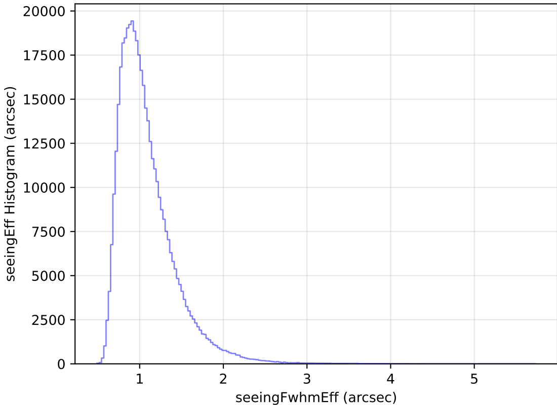
too_elab_r8_d3_giz_v3.4_10yrs WFD z band: seeingEff Histogram
