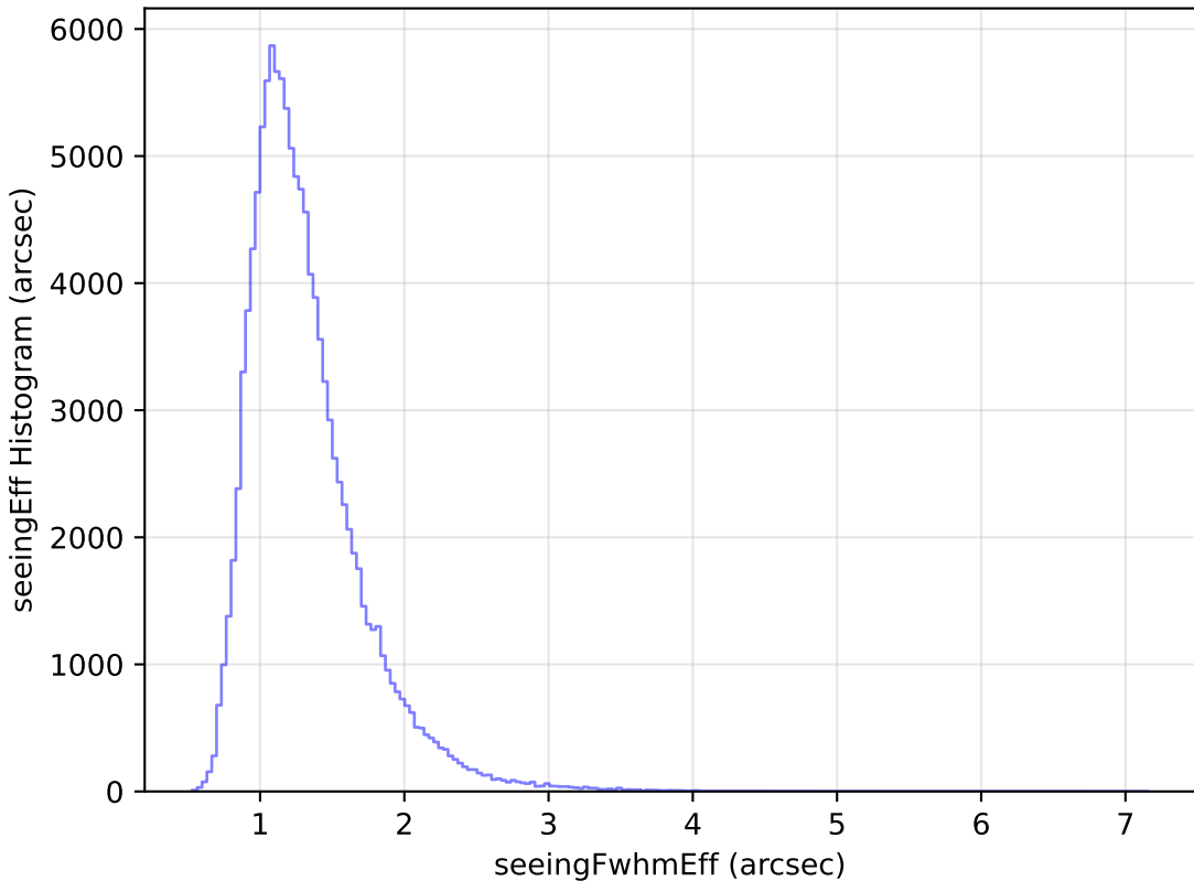
too_elab_r8_d3_giz_v3.4_10yrs WFD u band: seeingEff Histogram
