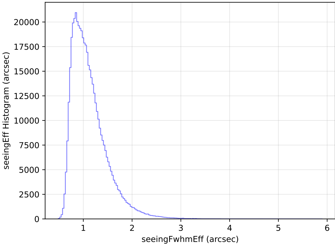
too_elab_r8_d3_giz_v3.4_10yrs WFD r band: seeingEff Histogram
