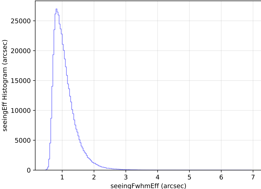
too_elab_r8_d3_giz_v3.4_10yrs WFD i band: seeingEff Histogram
