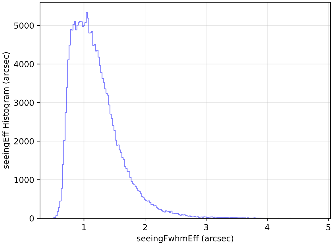
too_elab_r8_d3_giz_v3.4_10yrs WFD g band: seeingEff Histogram
