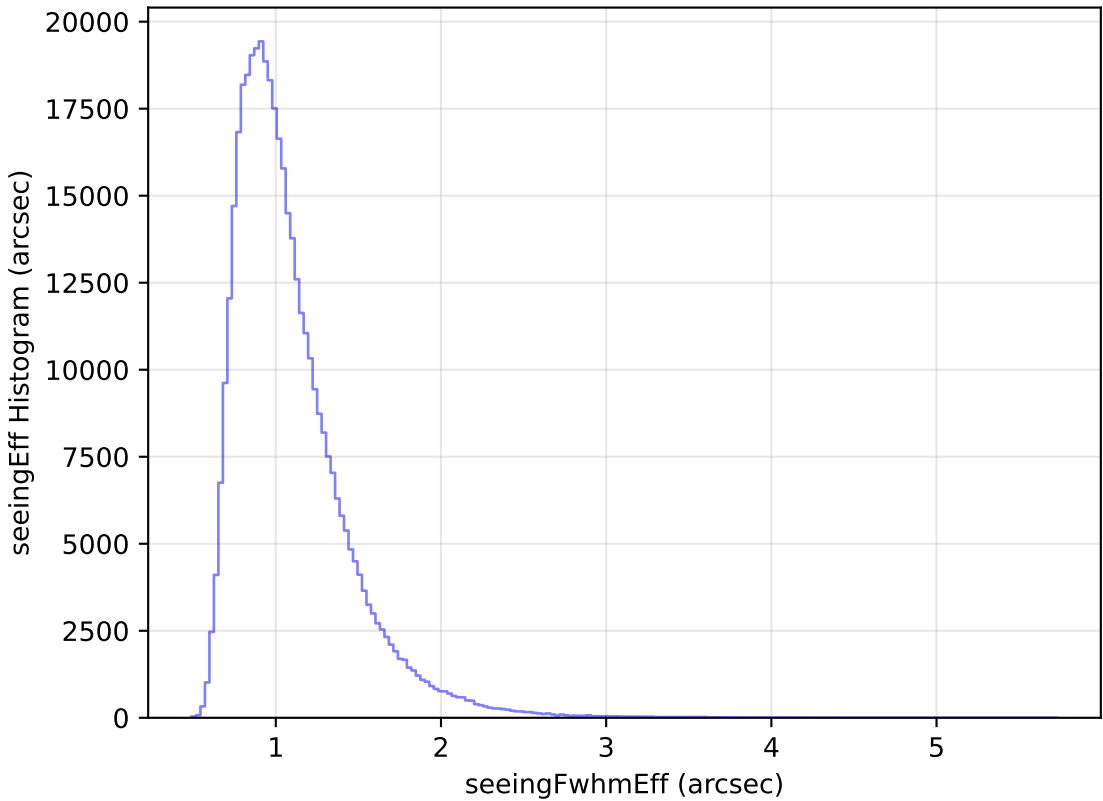
too_elab_r8_d3_giz_v3.4_10yrs All sky z band: seeingEff Histogram
