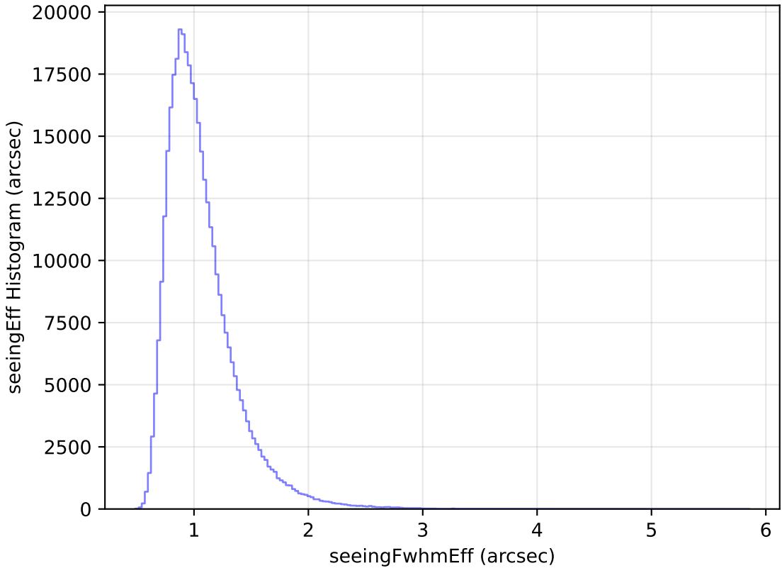
too_elab_r8_d3_giz_v3.4_10yrs All sky y band: seeingEff Histogram
