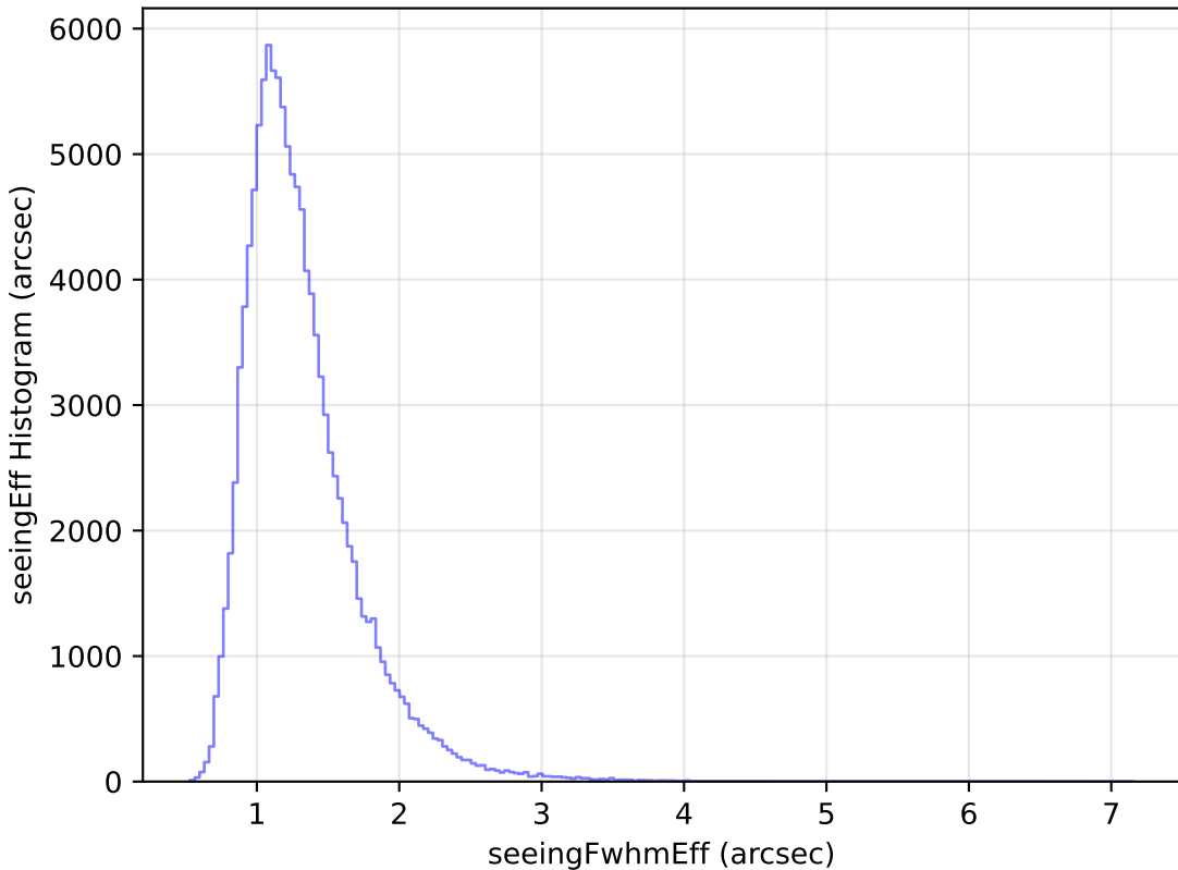
too_elab_r8_d3_giz_v3.4_10yrs All sky u band: seeingEff Histogram
