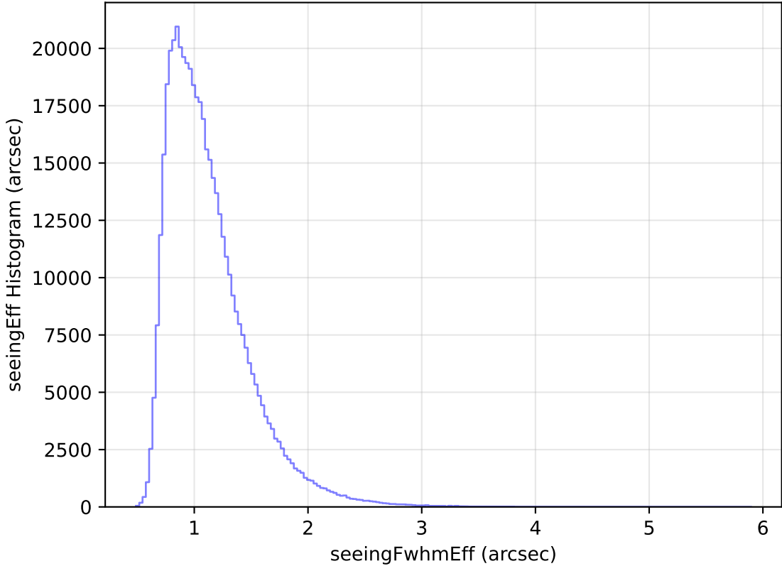
too_elab_r8_d3_giz_v3.4_10yrs All sky r band: seeingEff Histogram
