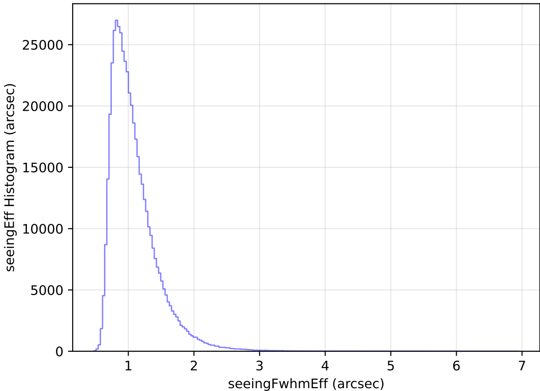
too_elab_r8_d3_giz_v3.4_10yrs All sky i band: seeingEff Histogram
