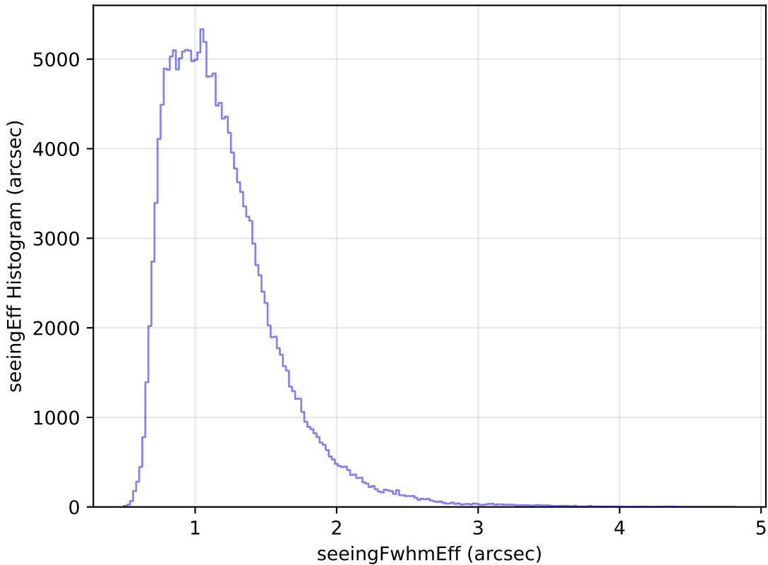
too_elab_r8_d3_giz_v3.4_10yrs All sky g band: seeingEff Histogram
