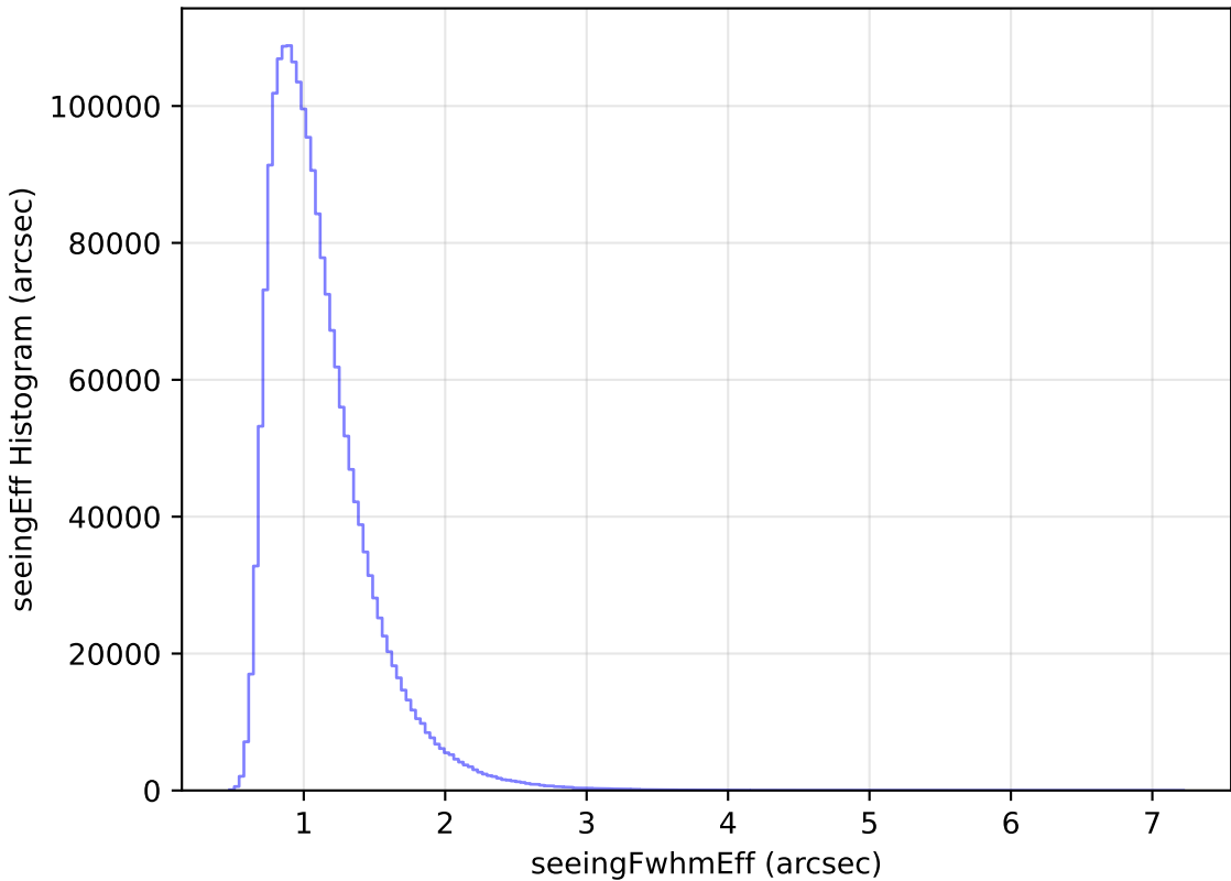
too_elab_r8_d3_giz_v3.4_10yrs All sky all bands: seeingEff Histogram
