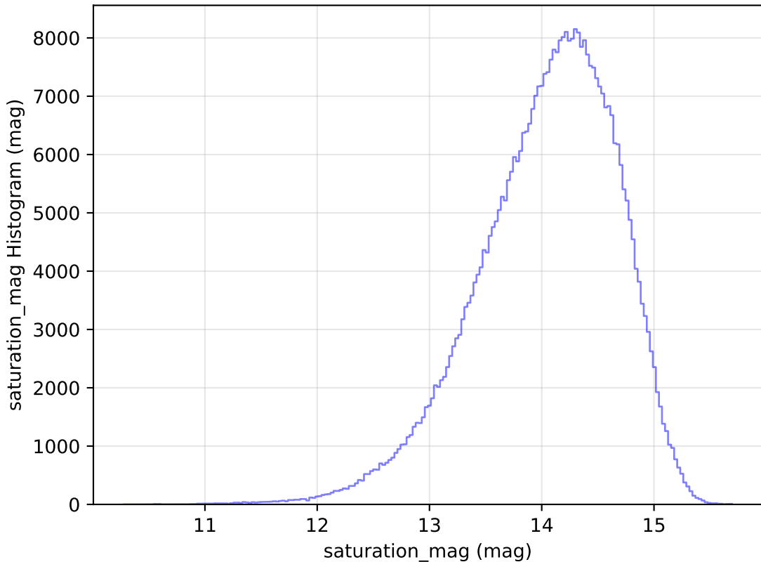
too_elab_r8_d3_giz_v3.4_10yrs WFD z band: saturation_mag Histogram
