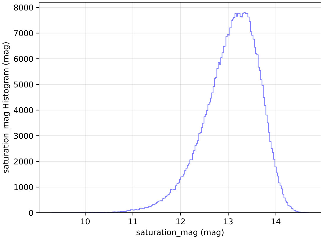
too_elab_r8_d3_giz_v3.4_10yrs WFD y band: saturation_mag Histogram
