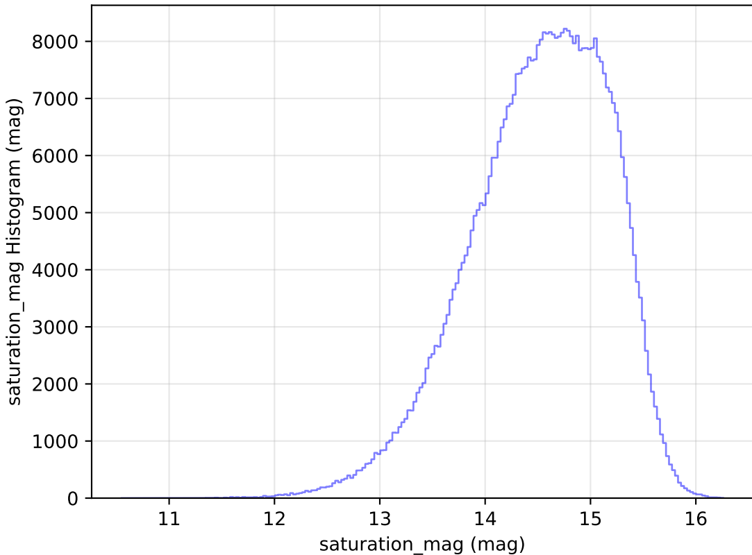
too_elab_r8_d3_giz_v3.4_10yrs WFD r band: saturation_mag Histogram
