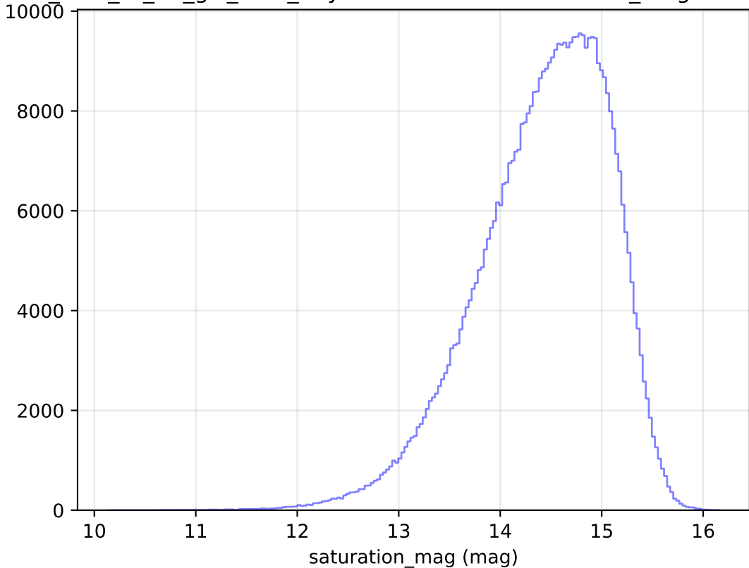
too_elab_r8_d3_giz_v3.4_10yrs WFD i band: saturation_mag Histogram
