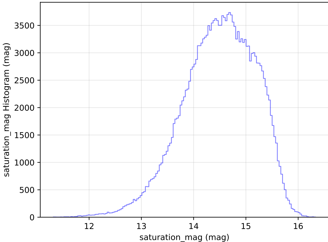
too_elab_r8_d3_giz_v3.4_10yrs WFD g band: saturation_mag Histogram
