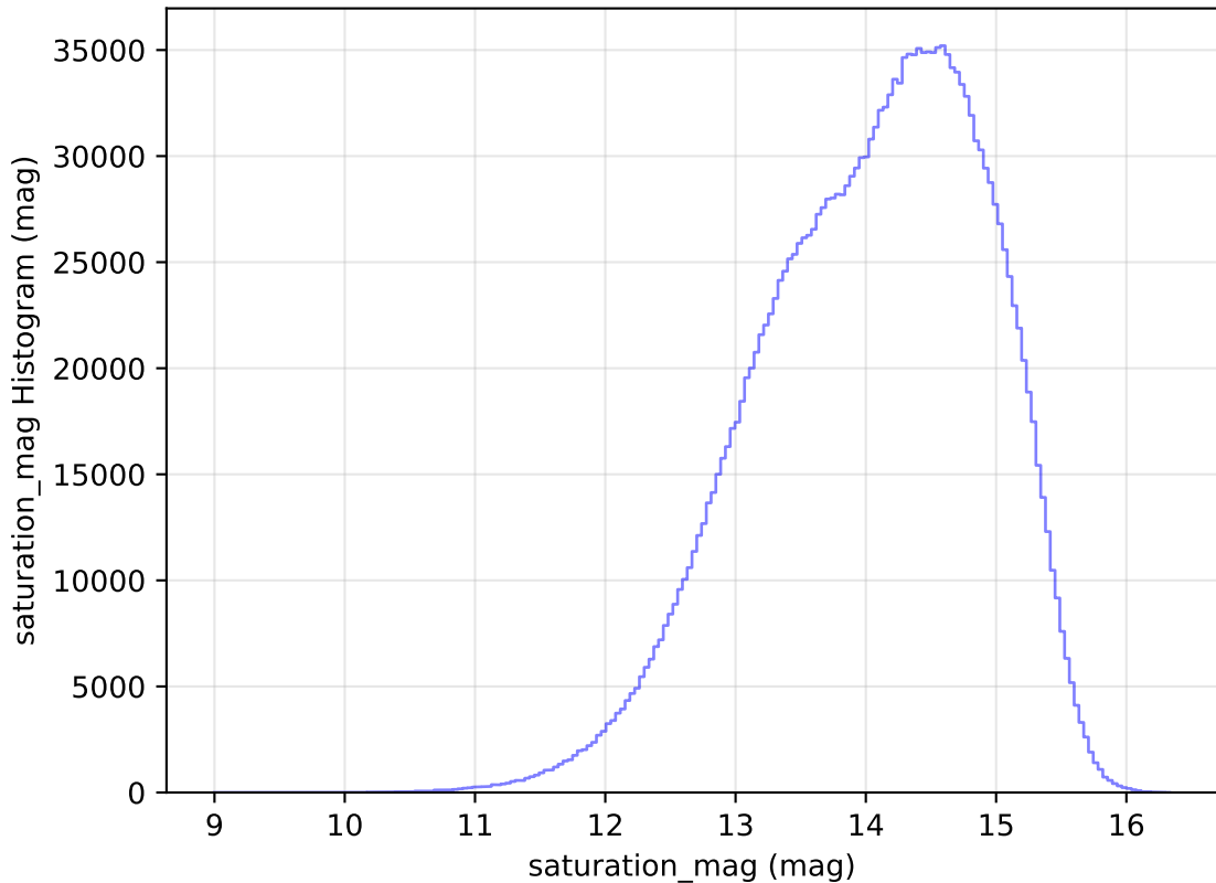
too_elab_r8_d3_giz_v3.4_10yrs WFD all bands: saturation_mag Histogram
