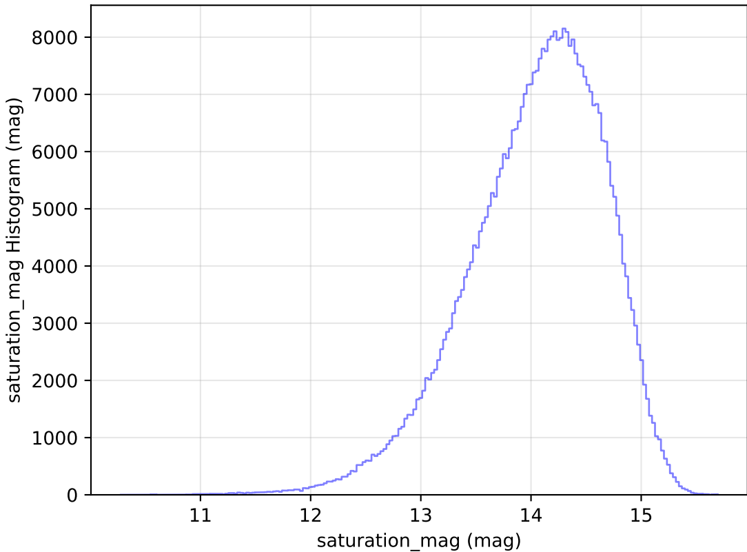
too_elab_r8_d3_giz_v3.4_10yrs All sky z band: saturation_mag Histogram
