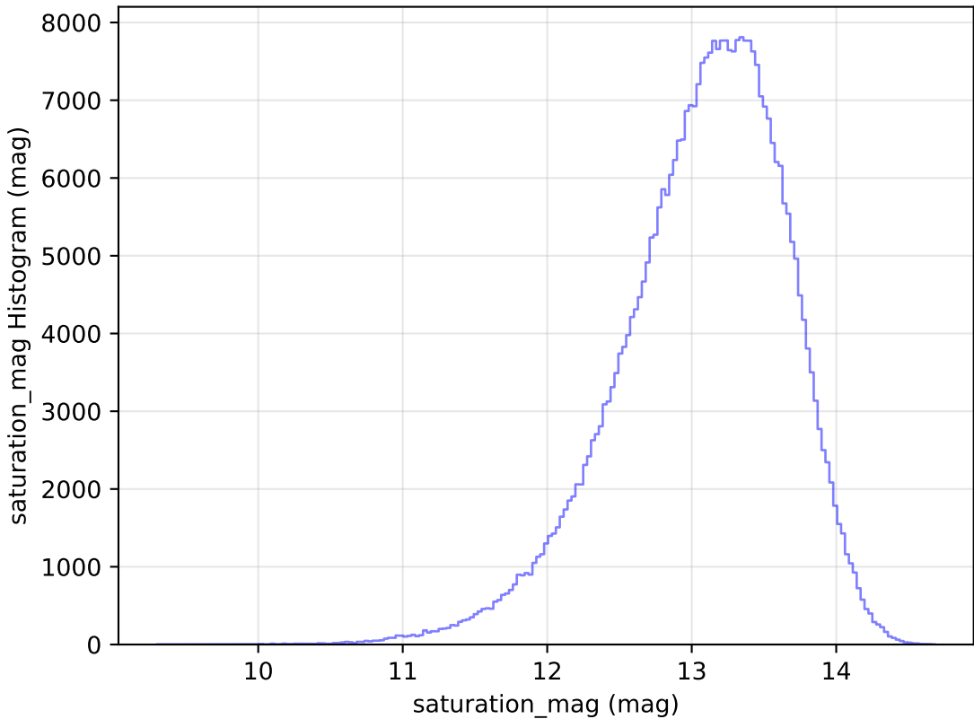
too_elab_r8_d3_giz_v3.4_10yrs All sky y band: saturation_mag Histogram
