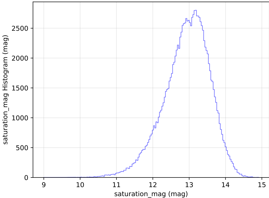
too_elab_r8_d3_giz_v3.4_10yrs All sky u band: saturation_mag Histogram
