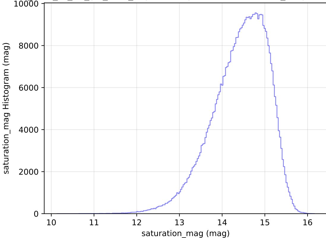
too_elab_r8_d3_giz_v3.4_10yrs All sky i band: saturation_mag Histogram
