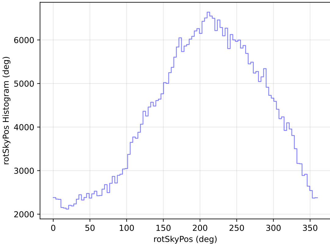
too_elab_r8_d3_giz_v3.4_10yrs WFD z band: rotSkyPos Histogram
