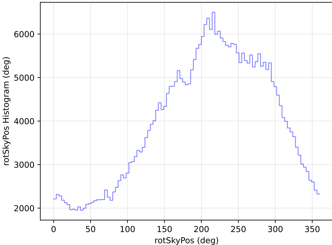
too_elab_r8_d3_giz_v3.4_10yrs WFD y band: rotSkyPos Histogram
