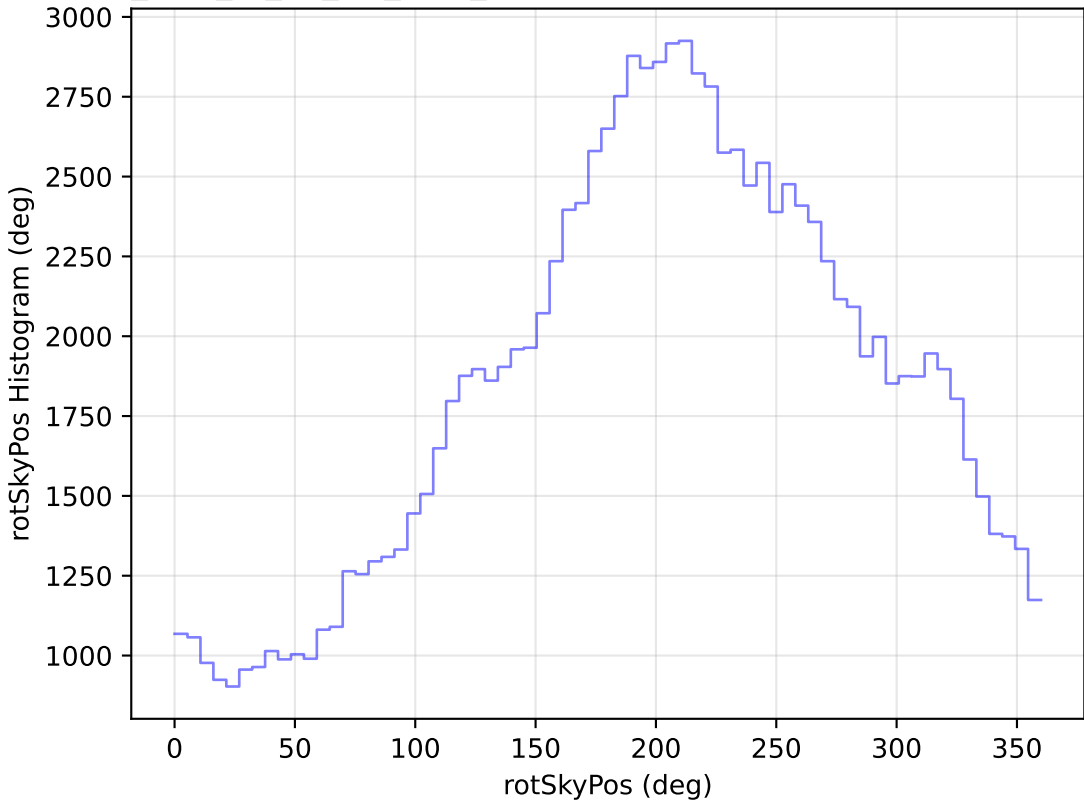
too_elab_r8_d3_giz_v3.4_10yrs WFD u band: rotSkyPos Histogram
