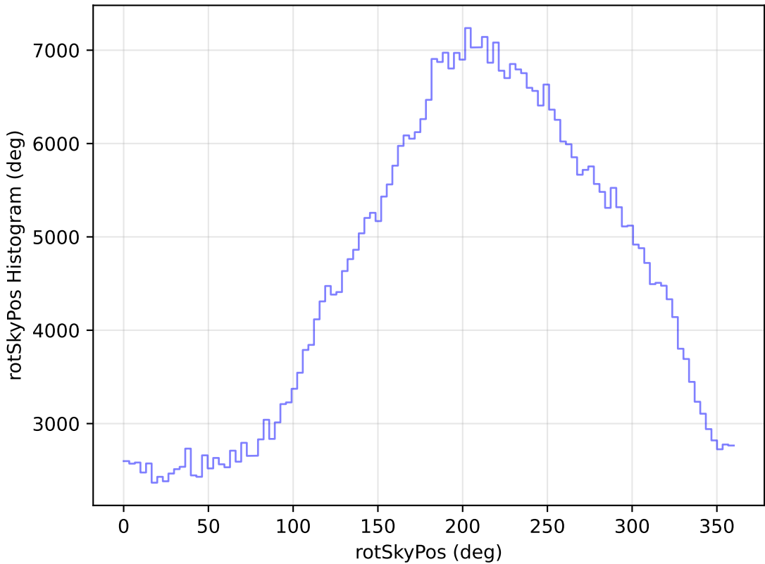
too_elab_r8_d3_giz_v3.4_10yrs WFD i band: rotSkyPos Histogram
