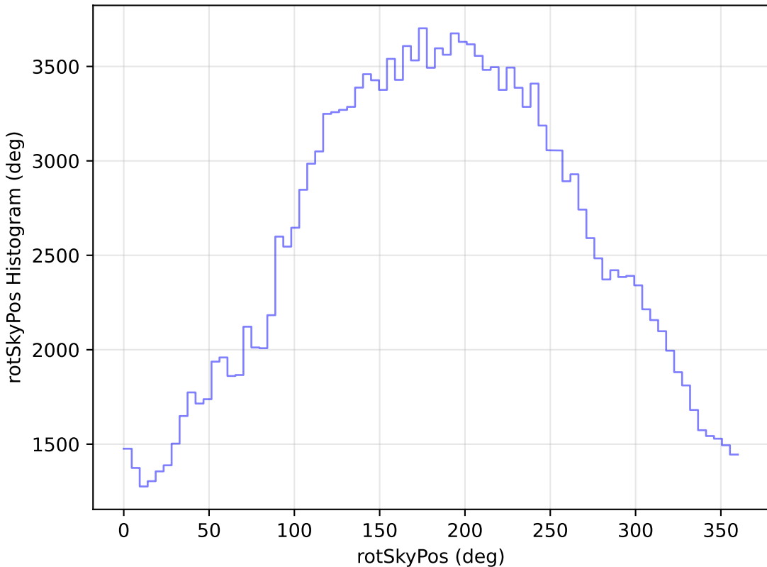
too_elab_r8_d3_giz_v3.4_10yrs WFD g band: rotSkyPos Histogram
