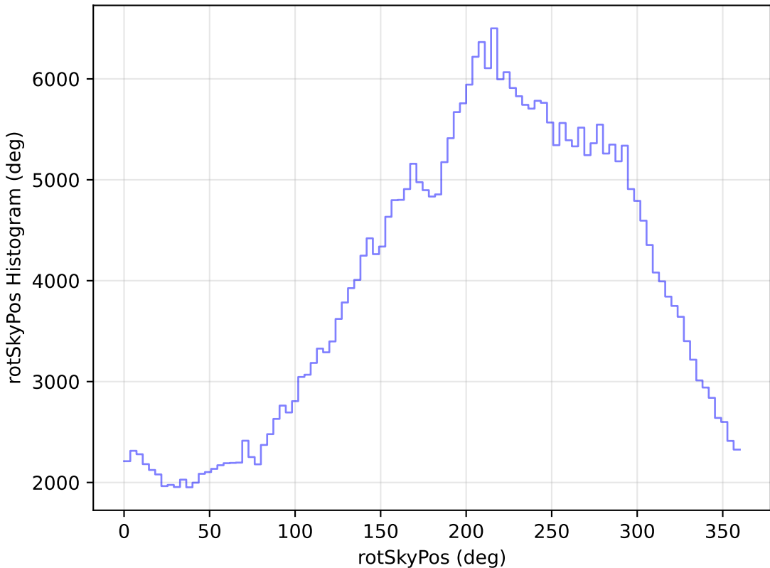
too_elab_r8_d3_giz_v3.4_10yrs All sky y band: rotSkyPos Histogram
