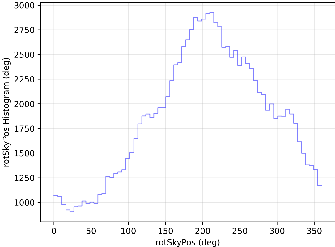
too_elab_r8_d3_giz_v3.4_10yrs All sky u band: rotSkyPos Histogram
