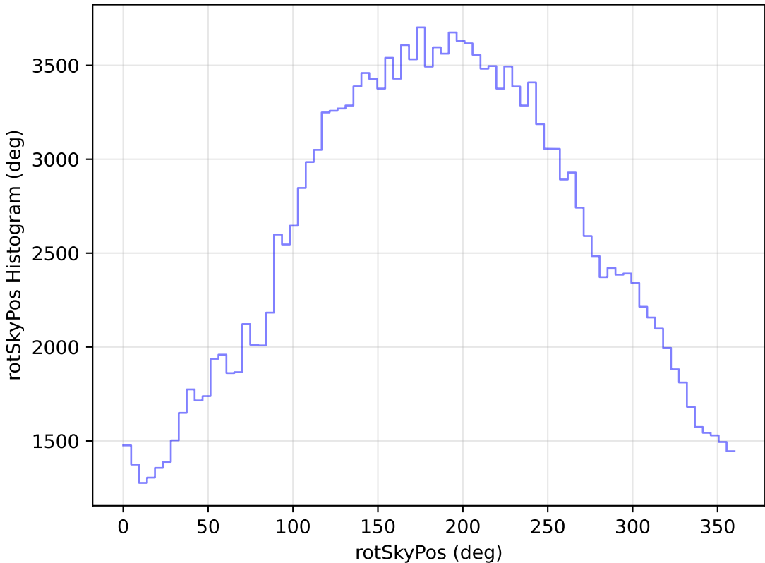
too_elab_r8_d3_giz_v3.4_10yrs All sky g band: rotSkyPos Histogram
