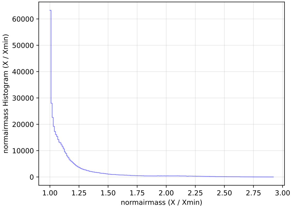
too_elab_r8_d3_giz_v3.4_10yrs WFD z band: normairmass Histogram
