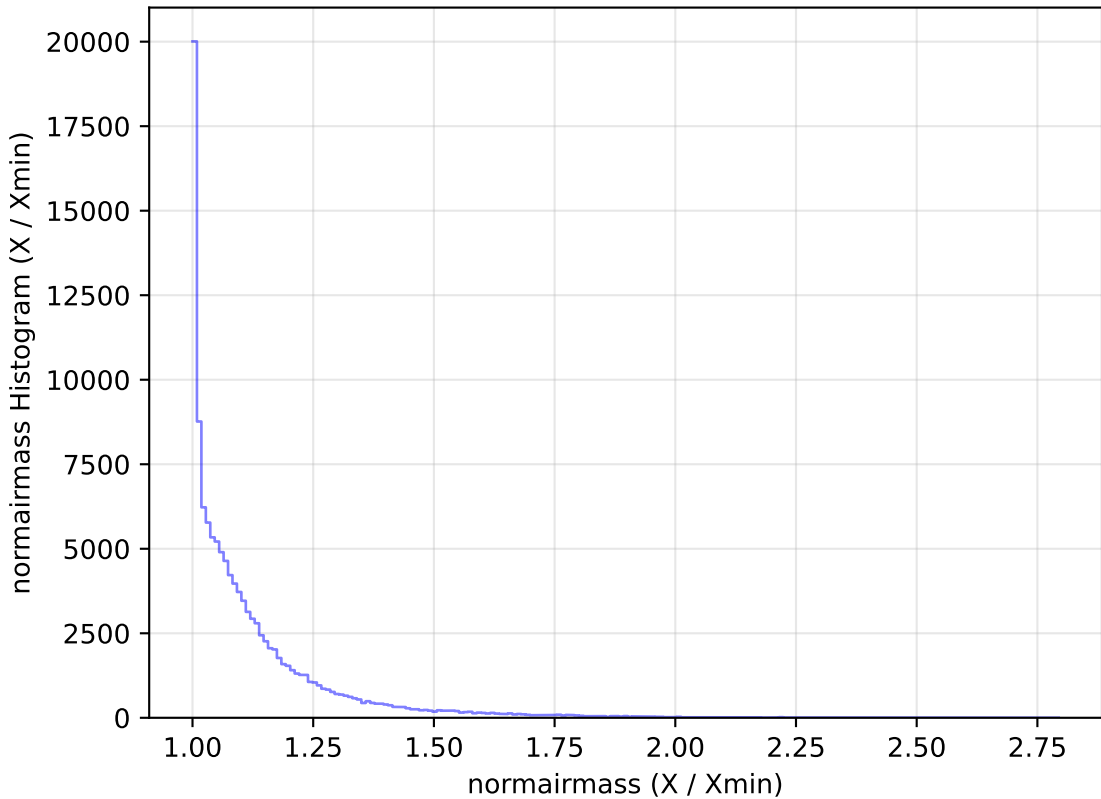
too_elab_r8_d3_giz_v3.4_10yrs WFD u band: normairmass Histogram
