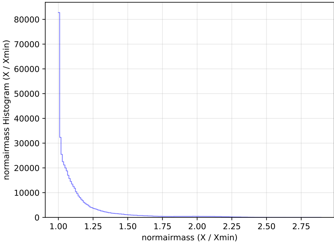
too_elab_r8_d3_giz_v3.4_10yrs WFD r band: normairmass Histogram
