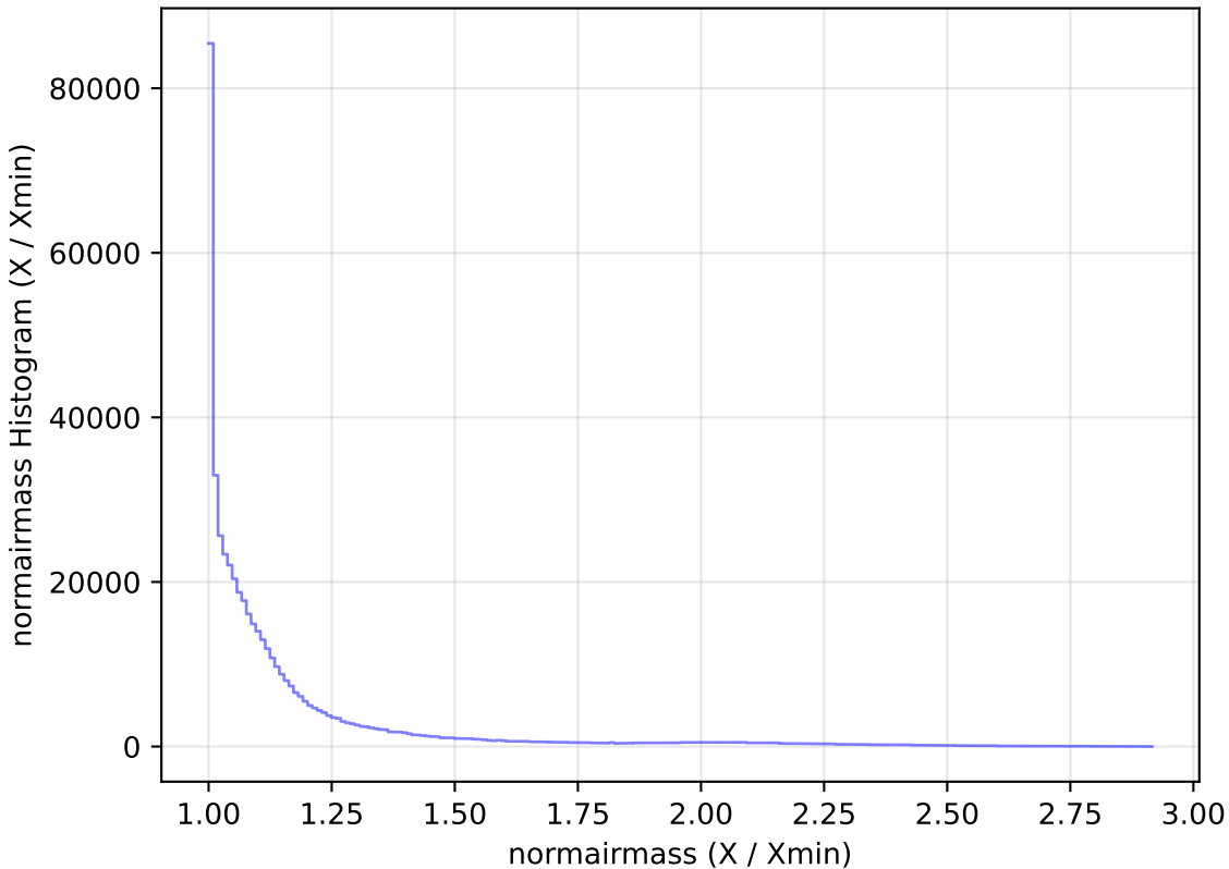
too_elab_r8_d3_giz_v3.4_10yrs WFD i band: normairmass Histogram
