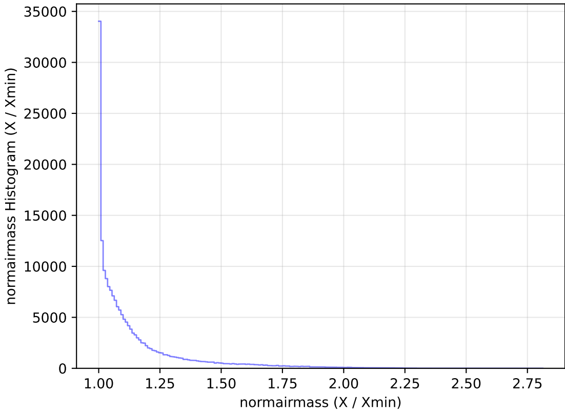
too_elab_r8_d3_giz_v3.4_10yrs WFD g band: normairmass Histogram
