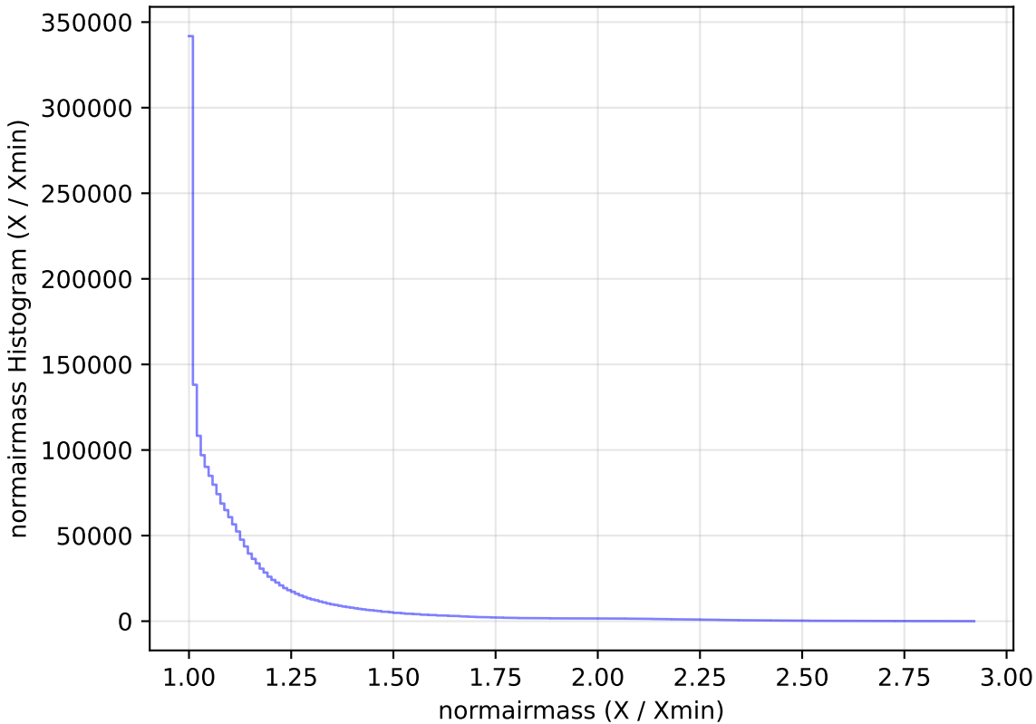
too_elab_r8_d3_giz_v3.4_10yrs WFD all bands: normairmass Histogram
