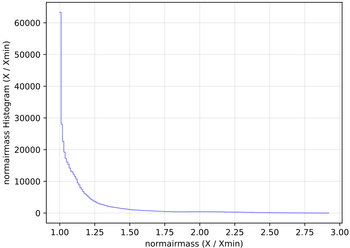
too_elab_r8_d3_giz_v3.4_10yrs All sky z band: normairmass Histogram
