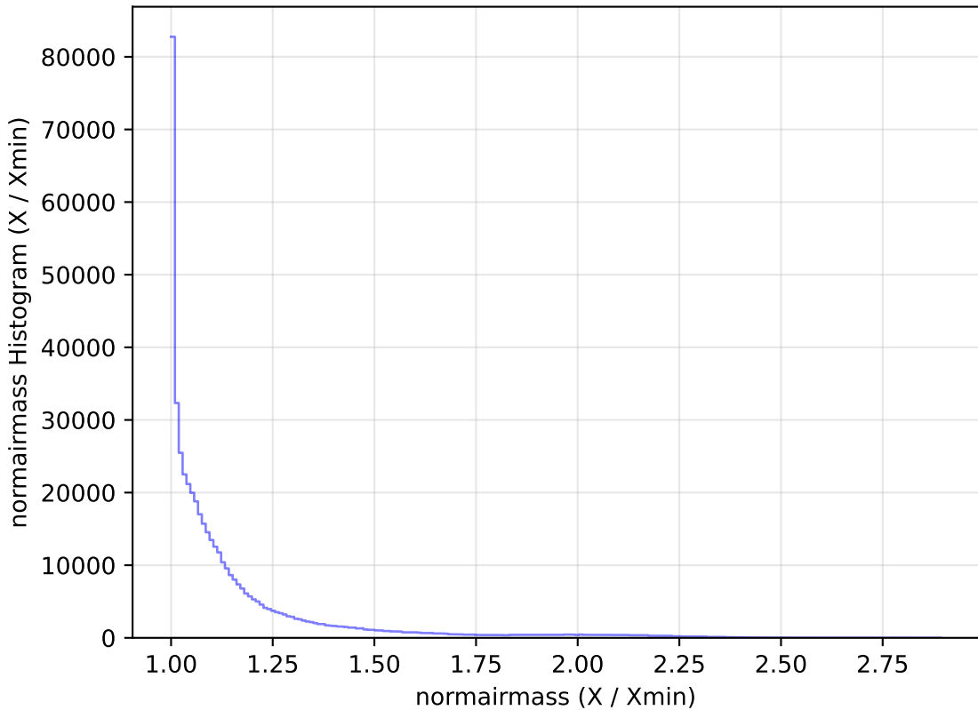
too_elab_r8_d3_giz_v3.4_10yrs All sky r band: normairmass Histogram
