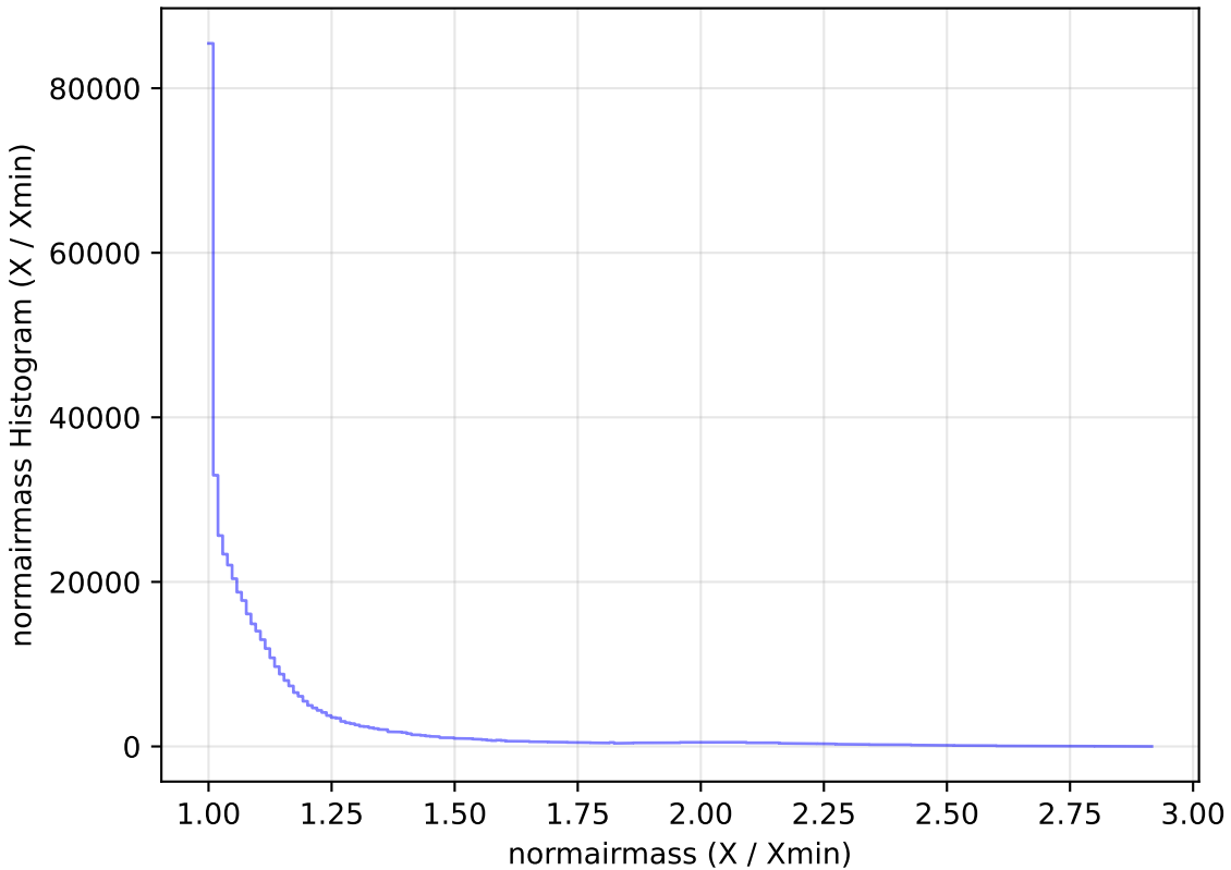
too_elab_r8_d3_giz_v3.4_10yrs All sky i band: normairmass Histogram
