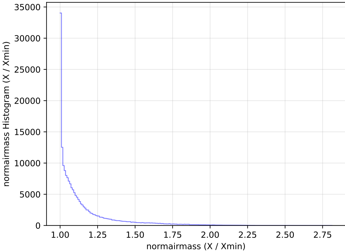
too_elab_r8_d3_giz_v3.4_10yrs All sky g band: normairmass Histogram
