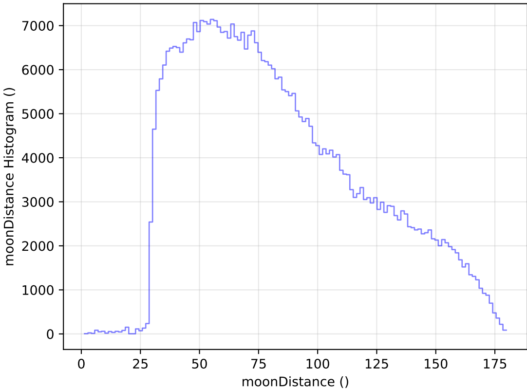
too_elab_r8_d3_giz_v3.4_10yrs WFD z band: moonDistance Histogram
